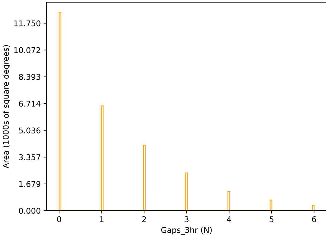
ddf_loaded_fl2_v3.4_10yrs r band: Gaps_3hr
