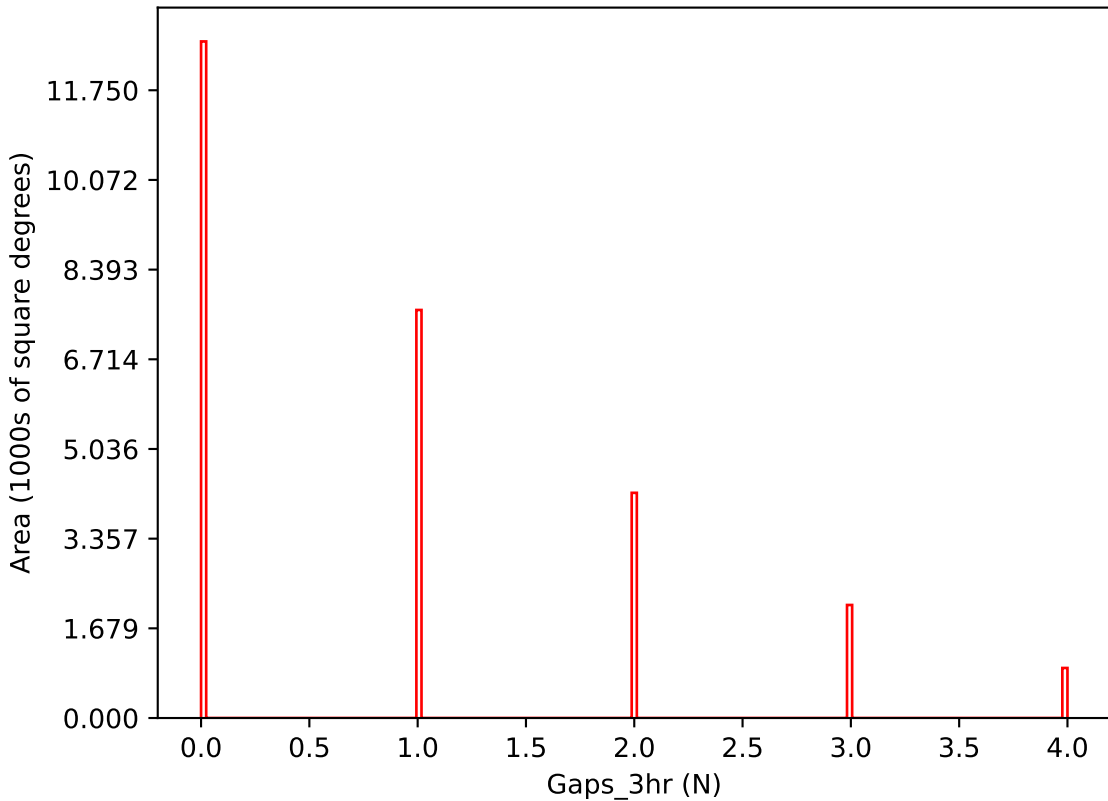
ddf_loaded_fl2_v3.4_10yrs i band: Gaps_3hr
