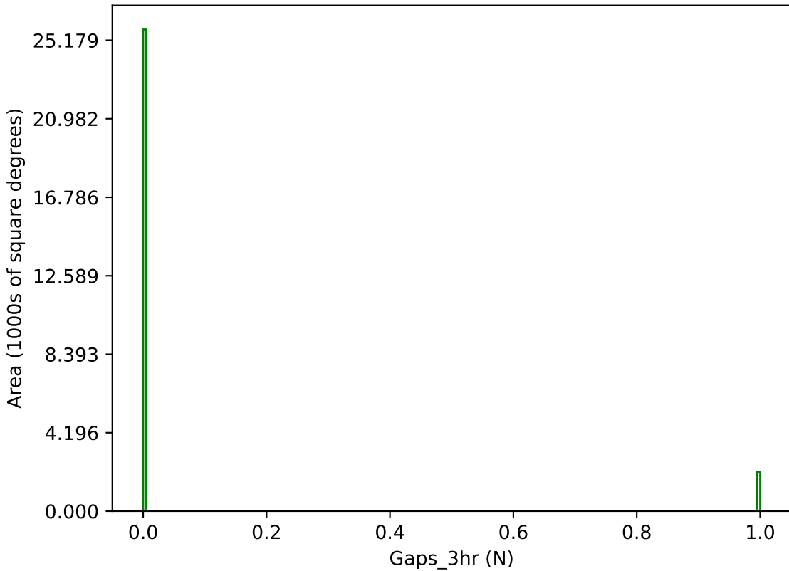
ddf_loaded_fl2_v3.4_10yrs g band: Gaps_3hr
