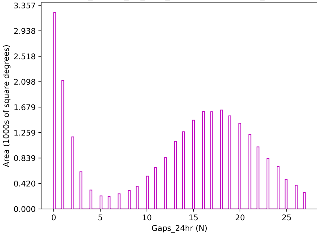
ddf_loaded_fl2_v3.4_10yrs z band: Gaps_24hr
