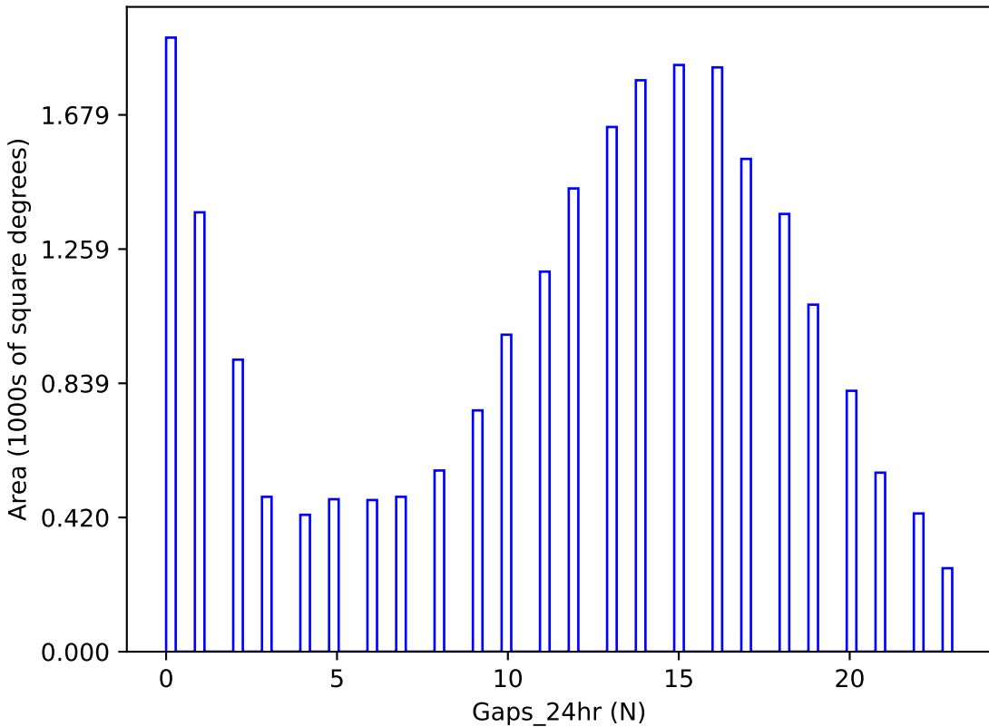
ddf_loaded_fl2_v3.4_10yrs y band: Gaps_24hr
