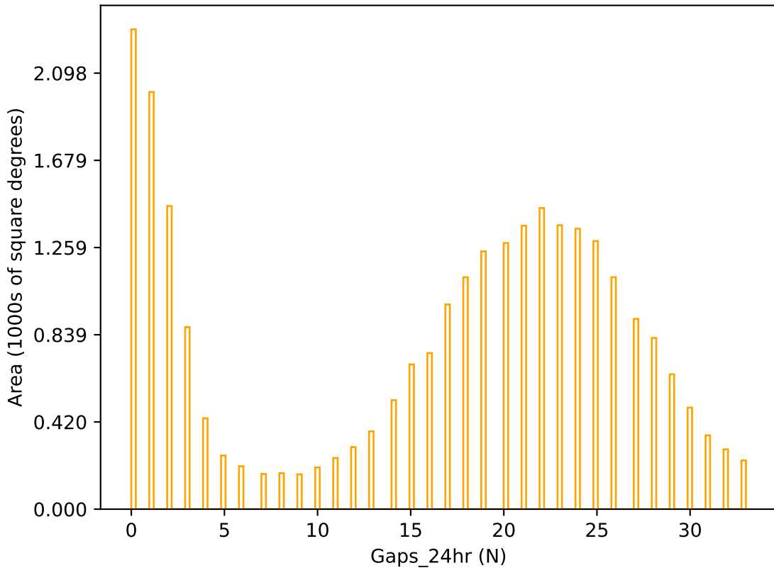
ddf_loaded_fl2_v3.4_10yrs r band: Gaps_24hr
