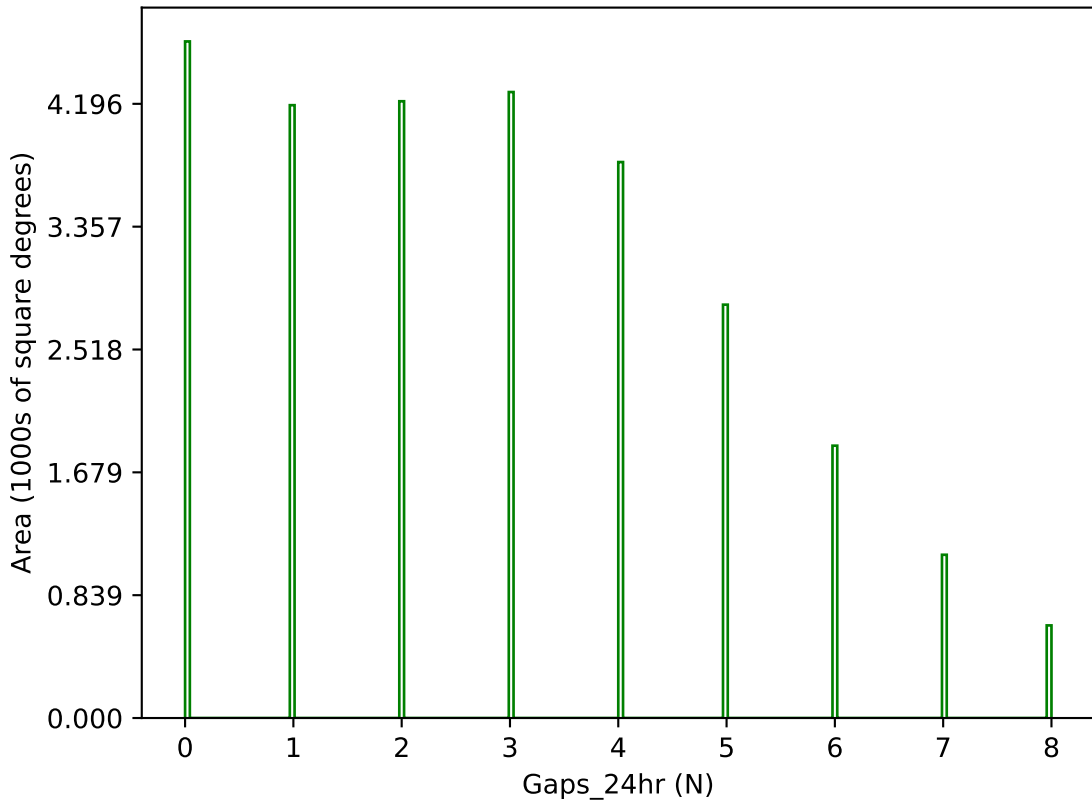
ddf_loaded_fl2_v3.4_10yrs g band: Gaps_24hr
