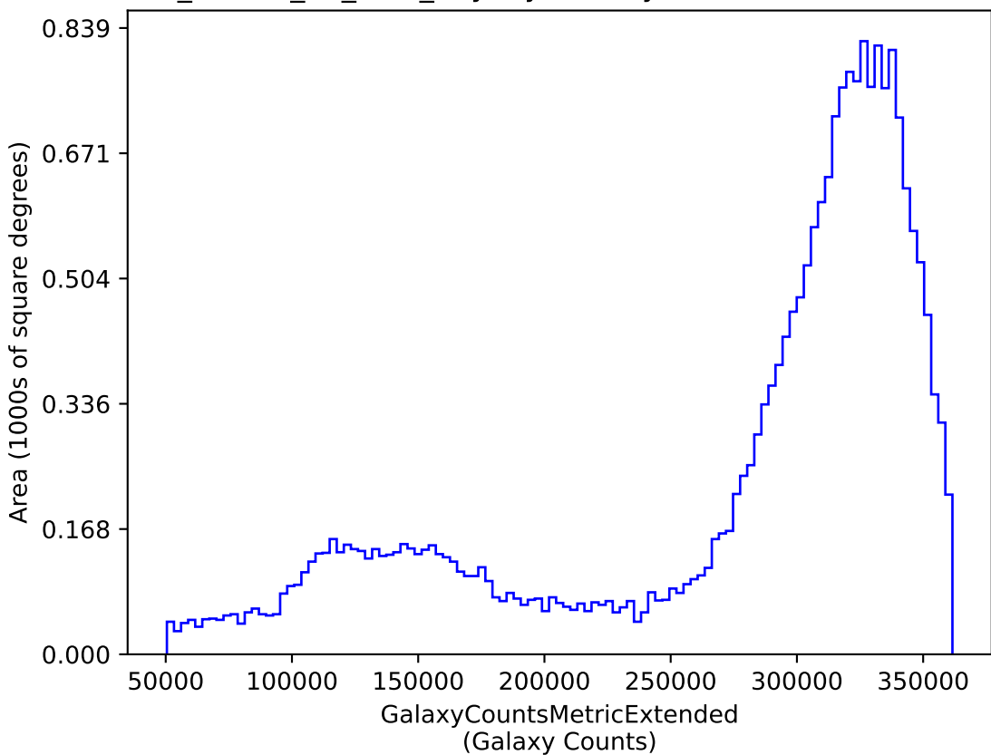
ddf_loaded_fl2_v3.4_10yrs y: GalaxyCountsMetricExtended
