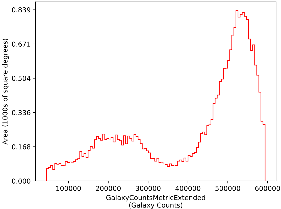
ddf_loaded_fl2_v3.4_10yrs i: GalaxyCountsMetricExtended
