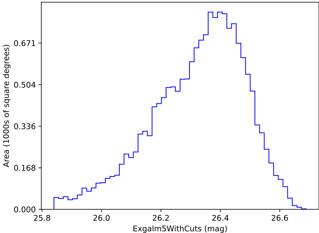
ddf_loaded_fl2_v3.4_10yrs i band non-DD year 9: ExgalM5WithCuts
