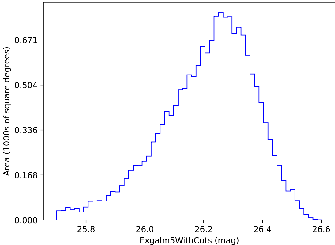
ddf_loaded_fl2_v3.4_10yrs i band non-DD year 7: ExgalM5WithCuts
