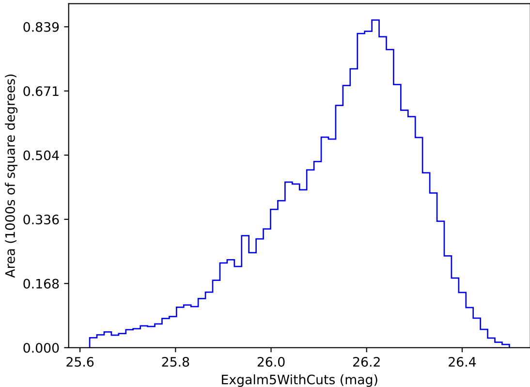
ddf_loaded_fl2_v3.4_10yrs i band non-DD year 6: ExgalM5WithCuts
