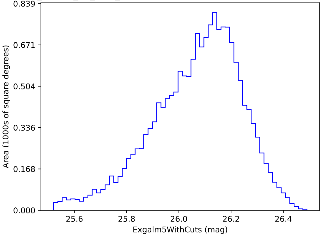
ddf_loaded_fl2_v3.4_10yrs i band non-DD year 5: Exgal5WithCuts
