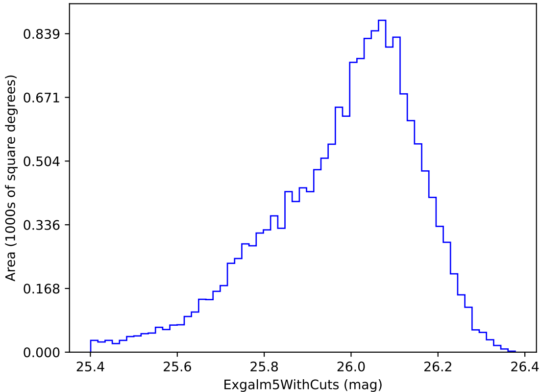
ddf_loaded_fl2_v3.4_10yrs i band non-DD year 4: ExgalM5WithCuts
