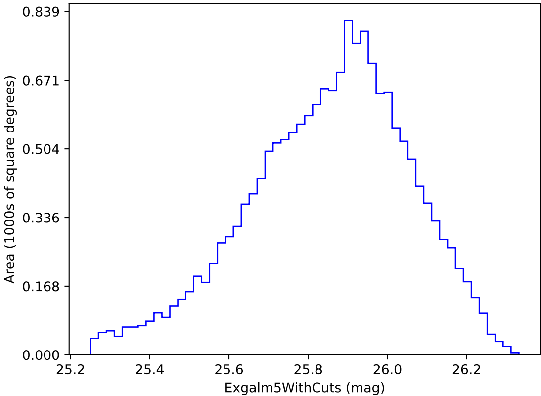
ddf_loaded_fl2_v3.4_10yrs i band non-DD year 3: ExgalM5WithCuts
