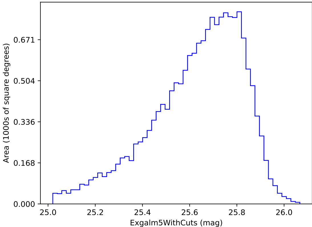
ddf_loaded_fl2_v3.4_10yrs i band non-DD year 2: ExgalM5WithCuts
