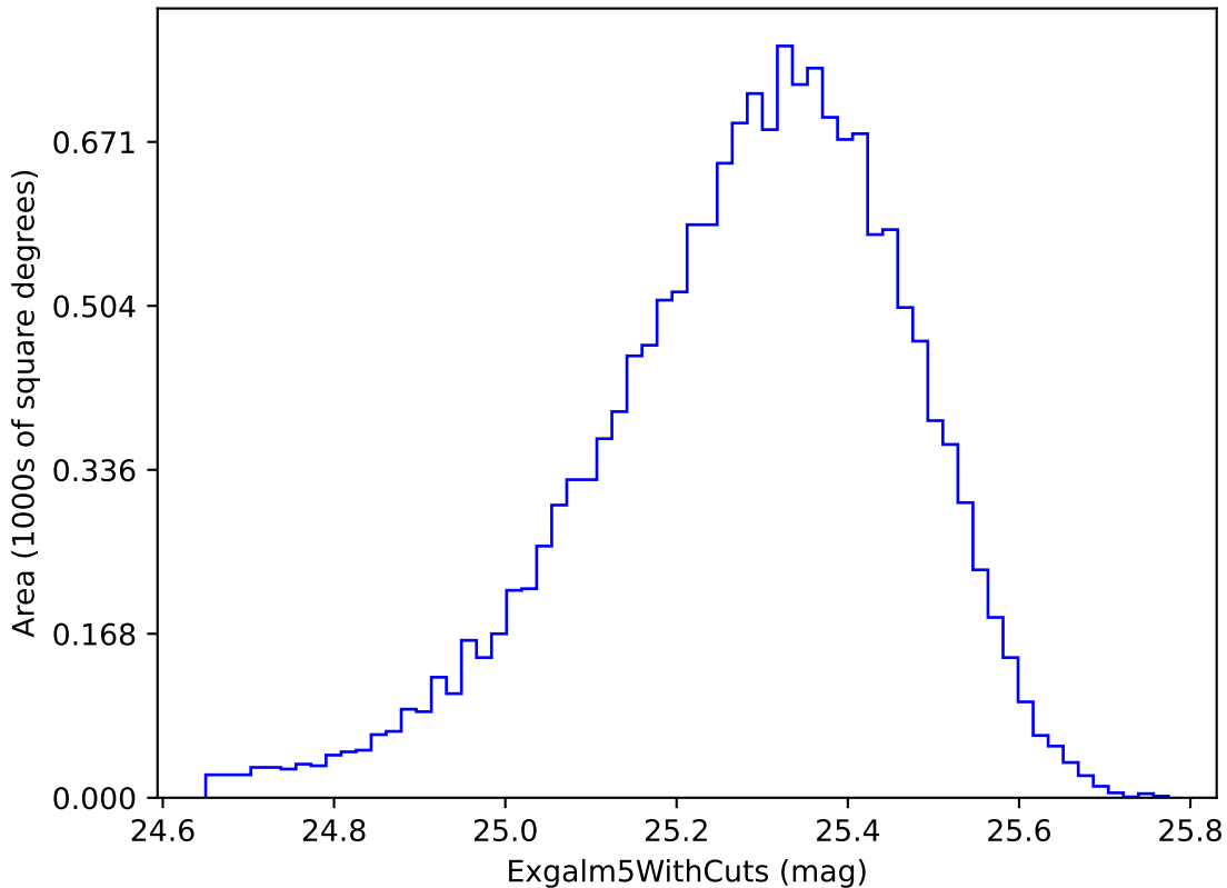
ddf_loaded_fl2_v3.4_10yrs i band non-DD year 1: ExgalM5WithCuts
