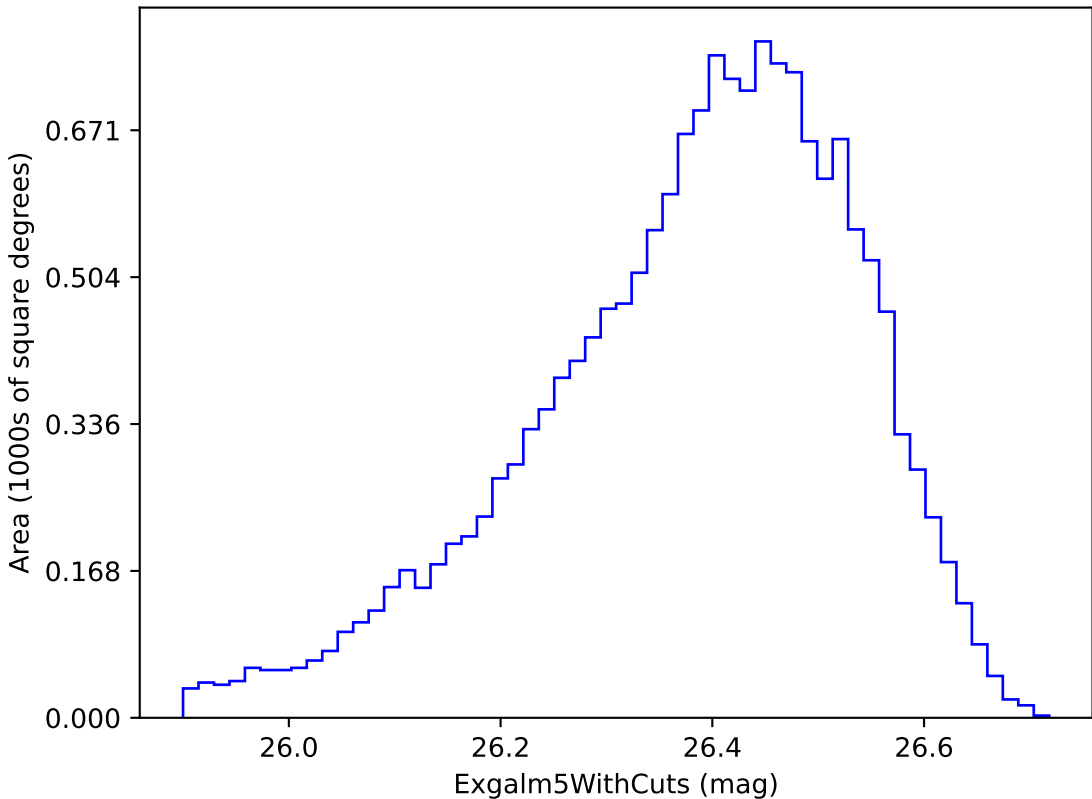
ddf_loaded_fl2_v3.4_10yrs i band non-DD year 10: ExgalM5WithCuts
