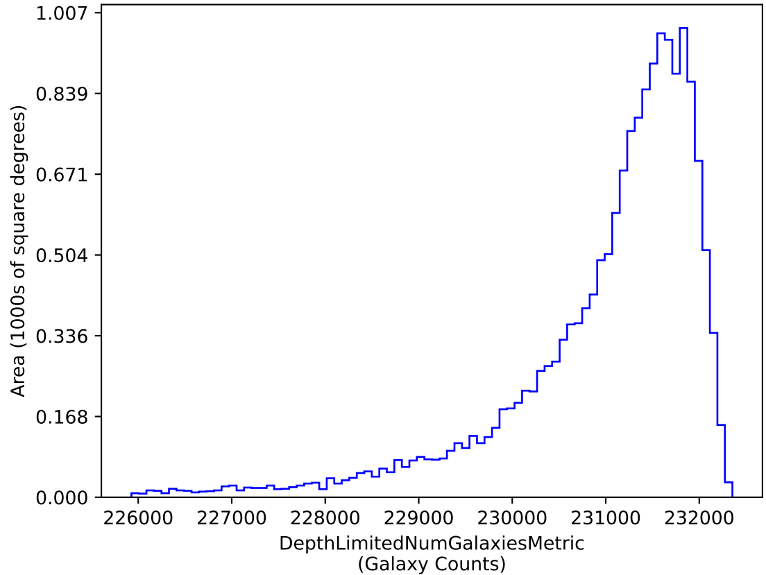
ddf_loaded_fl2_v3.4_10yrs i band galaxies non-DD: DepthLimitedNumGalaxiesMetric
