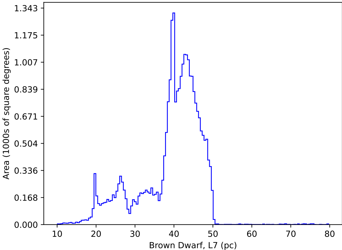
ddf_loaded_fl2_v3.4_10yrs : Brown Dwarf, L7
