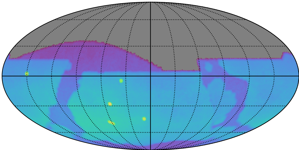
ddf_loaded_fl2_v3.4_10yrs : Brown Dwarf, L4
