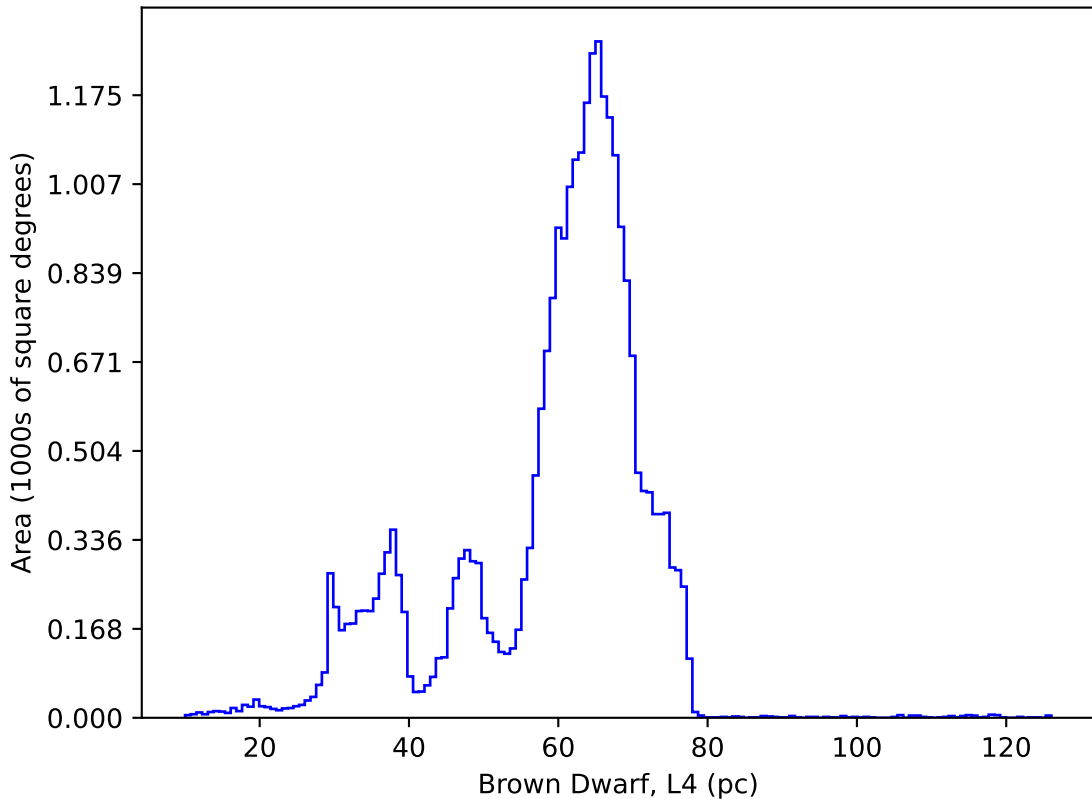
ddf_loaded_fl2_v3.4_10yrs : Brown Dwarf, L4
