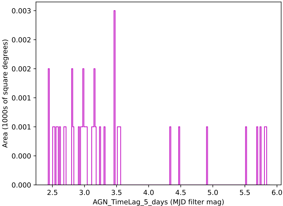
ddf_loaded_fl2_v3.4_10yrs z band: AGN_TimeLag_5_days
