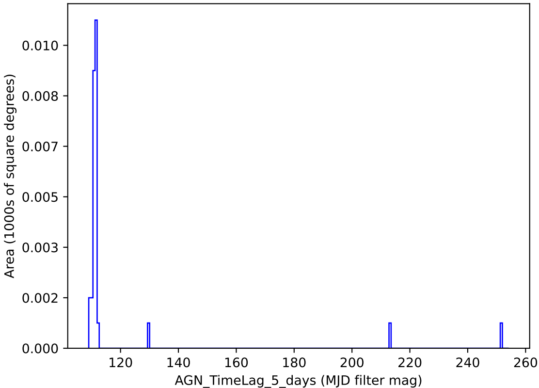
ddf_loaded_fl2_v3.4_10yrs y band: AGN_TimeLag_5_days
