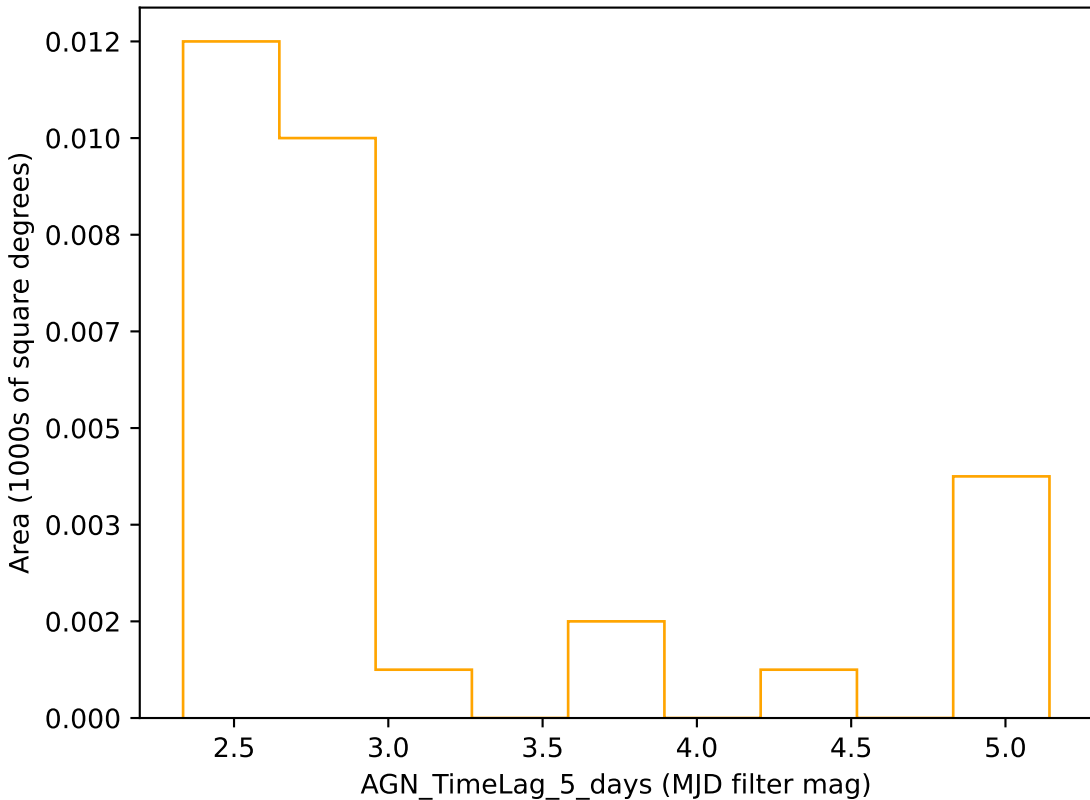
ddf_loaded_fl2_v3.4_10yrs r band: AGN_TimeLag_5_days
