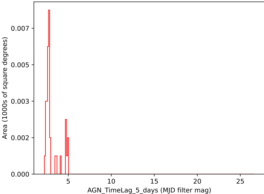
ddf_loaded_fl2_v3.4_10yrs i band: AGN_TimeLag_5_days
