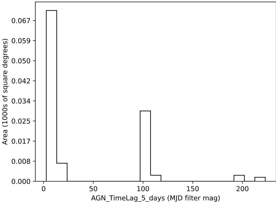
ddf_loaded_fl2_v3.4_10yrs all bands: AGN_TimeLag_5_days
