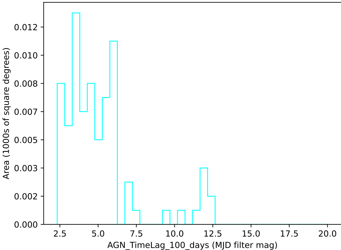
ddf_loaded_fl2_v3.4_10yrs u band: AGN_TimeLag_100_days
