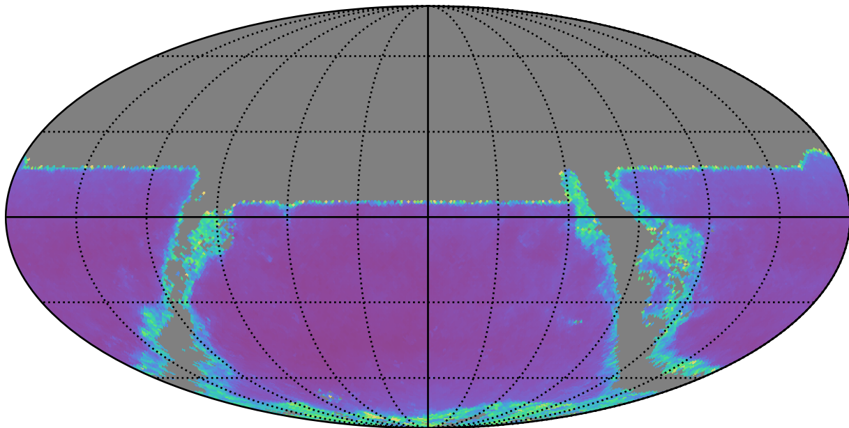
ddf_loaded_fl2_v3.4_10yrs y band: AGN SF_uncert
