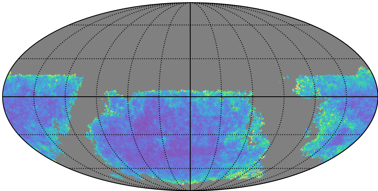
ddf_loaded_fl2_v3.4_10yrs u band: AGN SF_uncert
