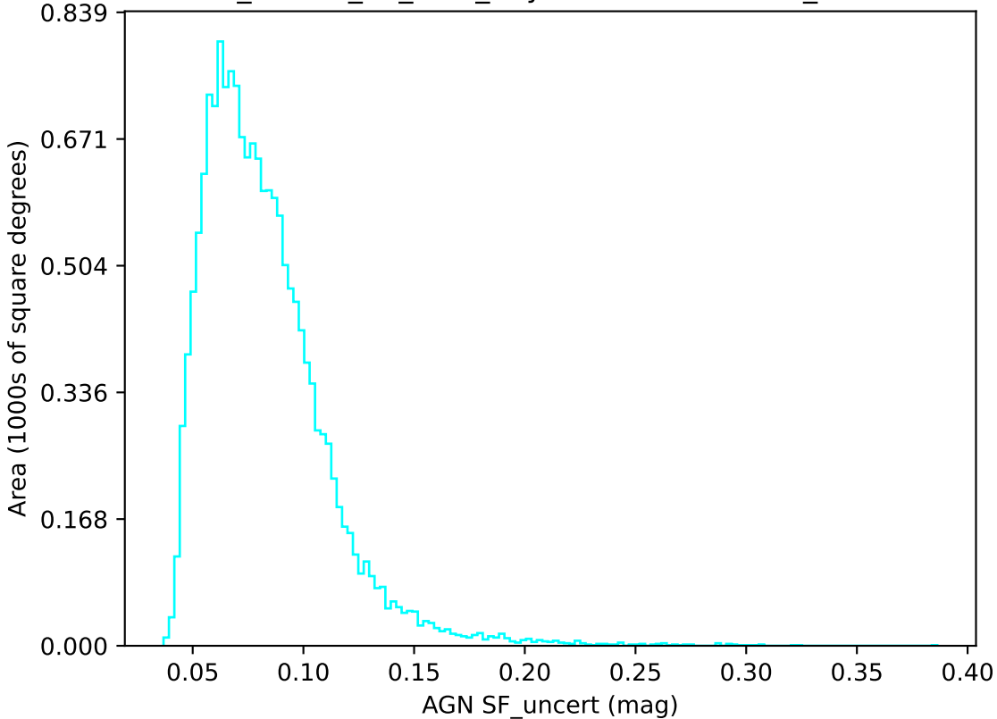
ddf_loaded_fl2_v3.4_10yrs u band: AGN SF_uncert
