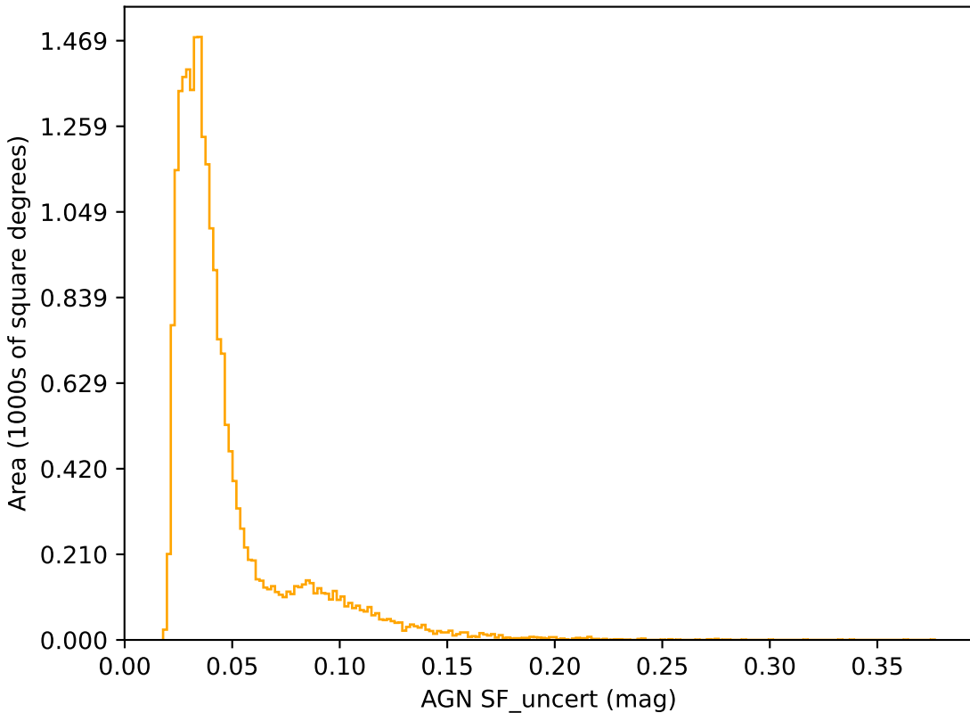
ddf_loaded_fl2_v3.4_10yrs r band: AGN SF_uncert
