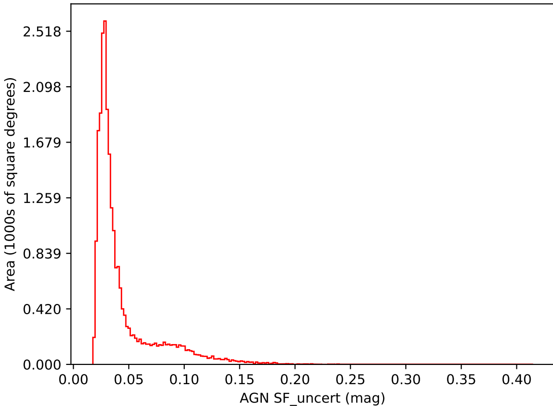
ddf_loaded_fl2_v3.4_10yrs i band: AGN SF_uncert
