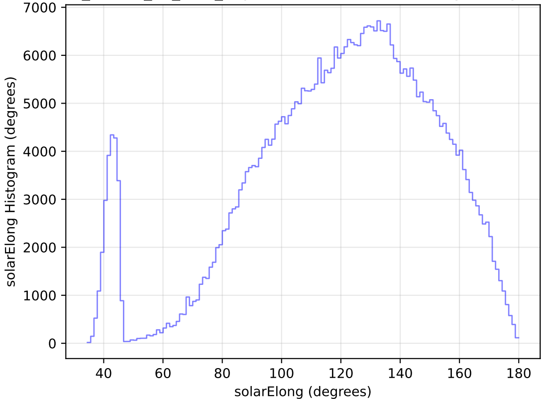
ddf_loaded_fl2_v3.4_10yrs WFD z band: solarElong Histogram
