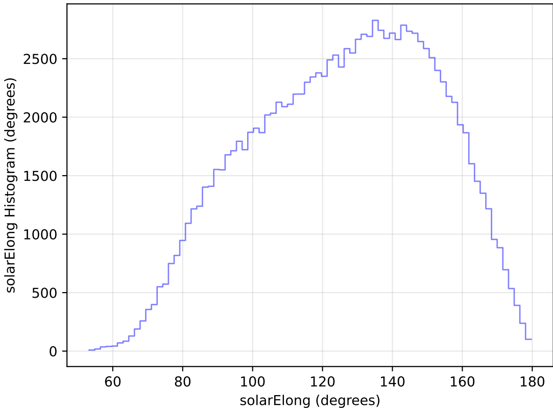
ddf_loaded_fl2_v3.4_10yrs WFD u band: solarElong Histogram
