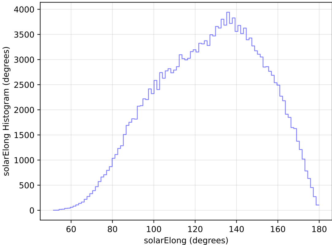
ddf_loaded_fl2_v3.4_10yrs WFD g band: solarElong Histogram
