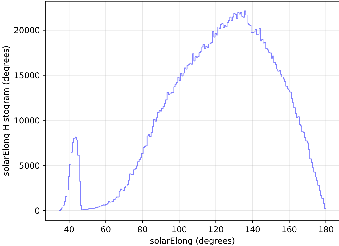
ddf_loaded_fl2_v3.4_10yrs WFD all bands: solarElong Histogram
