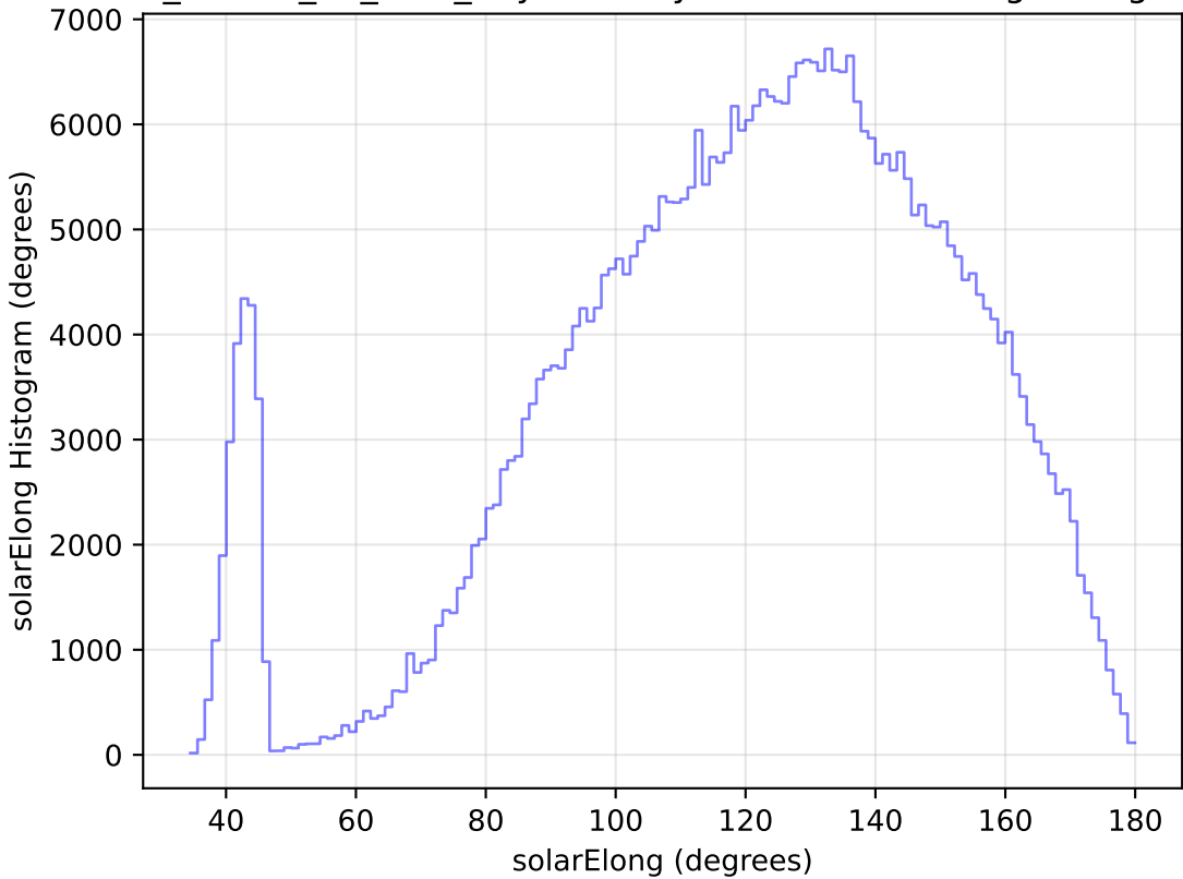
ddf_loaded_fl2_v3.4_10yrs All sky z band: solarElong Histogram
