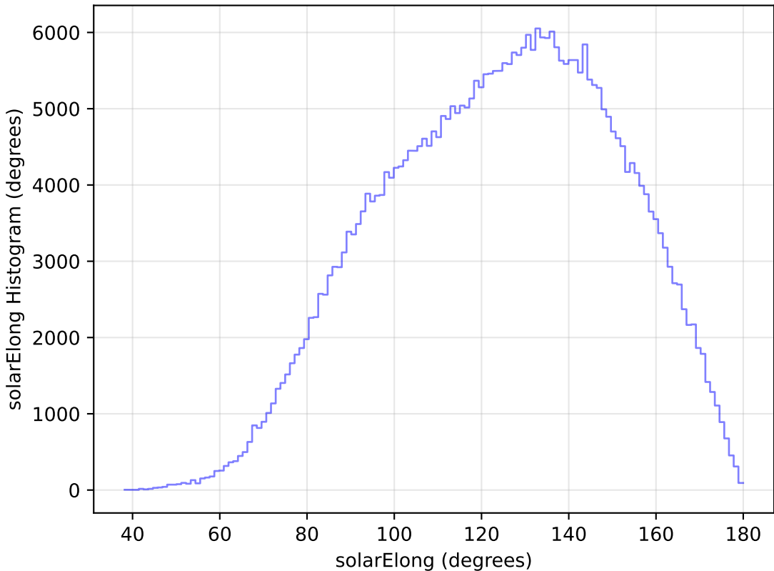
ddf_loaded_fl2_v3.4_10yrs All sky y band: solarElong Histogram
