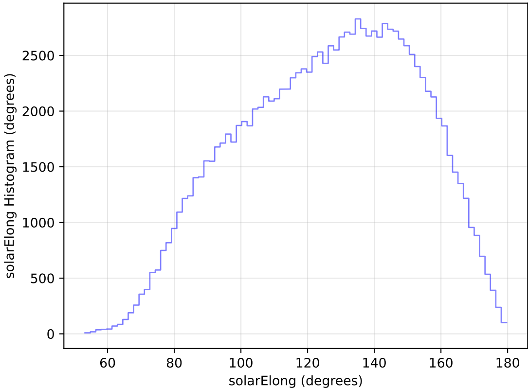
ddf_loaded_fl2_v3.4_10yrs All sky u band: solarElong Histogram
