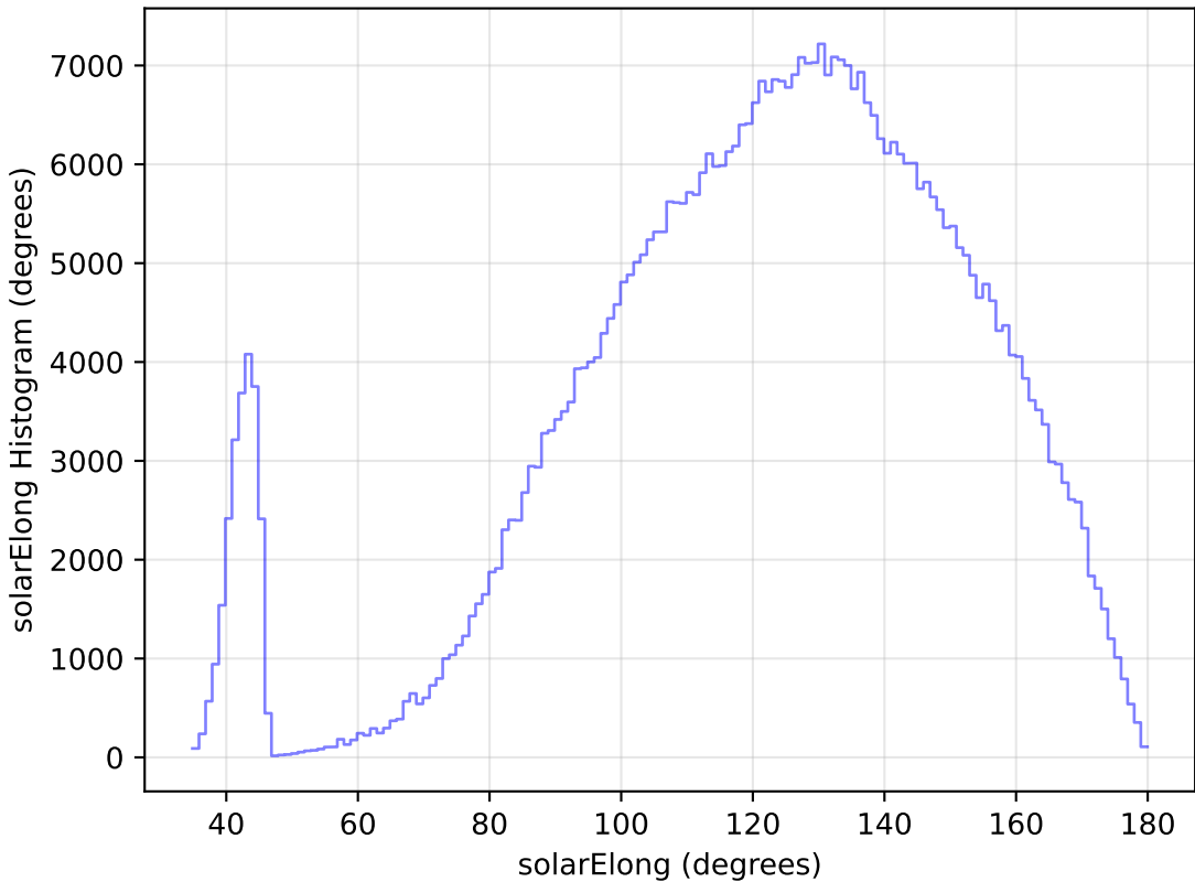
ddf_loaded_fl2_v3.4_10yrs All sky i band: solarElong Histogram
