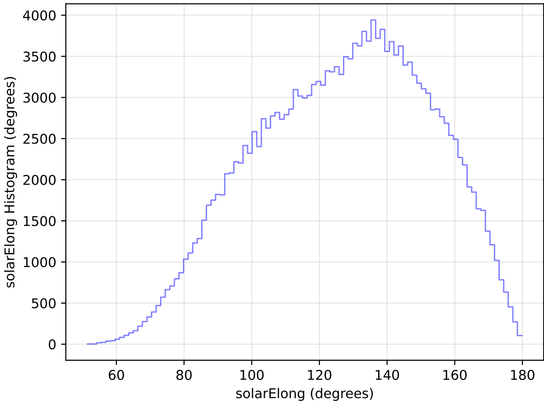
ddf_loaded_fl2_v3.4_10yrs All sky g band: solarElong Histogram
