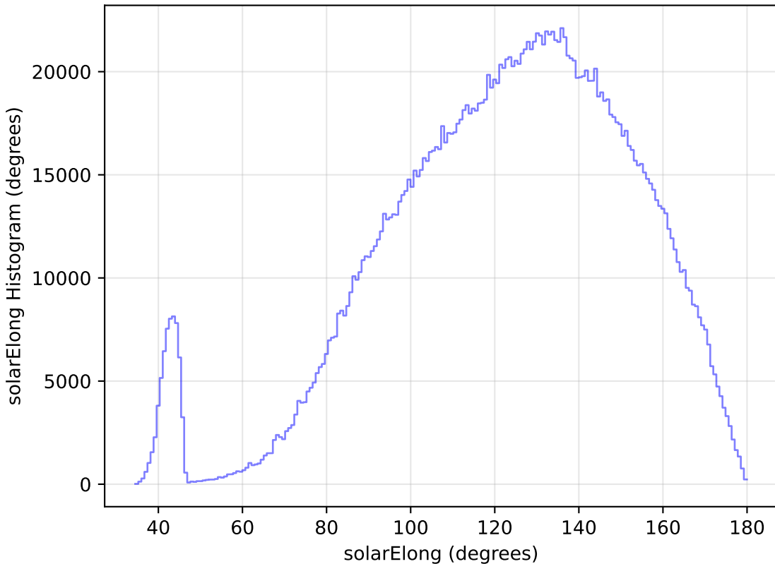
ddf_loaded_fl2_v3.4_10yrs All sky all bands: solarElong Histogram
