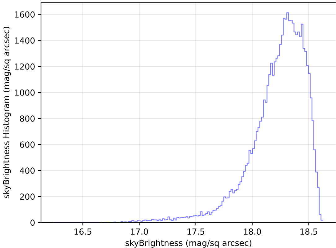
ddf_loaded_fl2_v3.4_10yrs Yr 1 y band: skyBrightness Histogram
