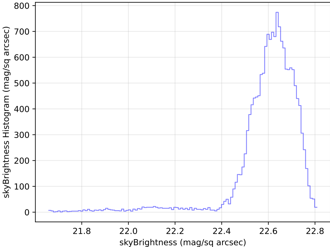
ddf_loaded_fl2_v3.4_10yrs Yr 1 u band: skyBrightness Histogram
