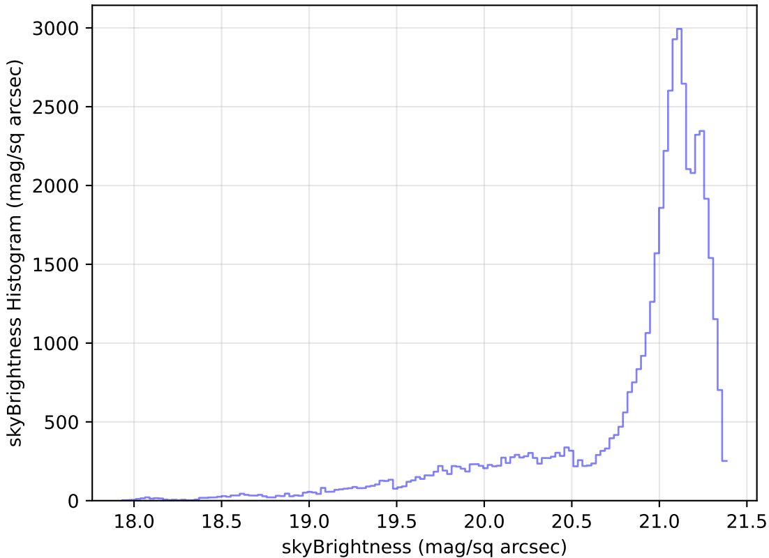
ddf_loaded_fl2_v3.4_10yrs Yr 1 r band: skyBrightness Histogram
