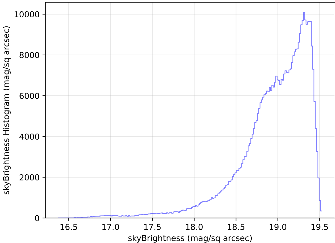
ddf_loaded_fl2_v3.4_10yrs WFD z band: skyBrightness Histogram
