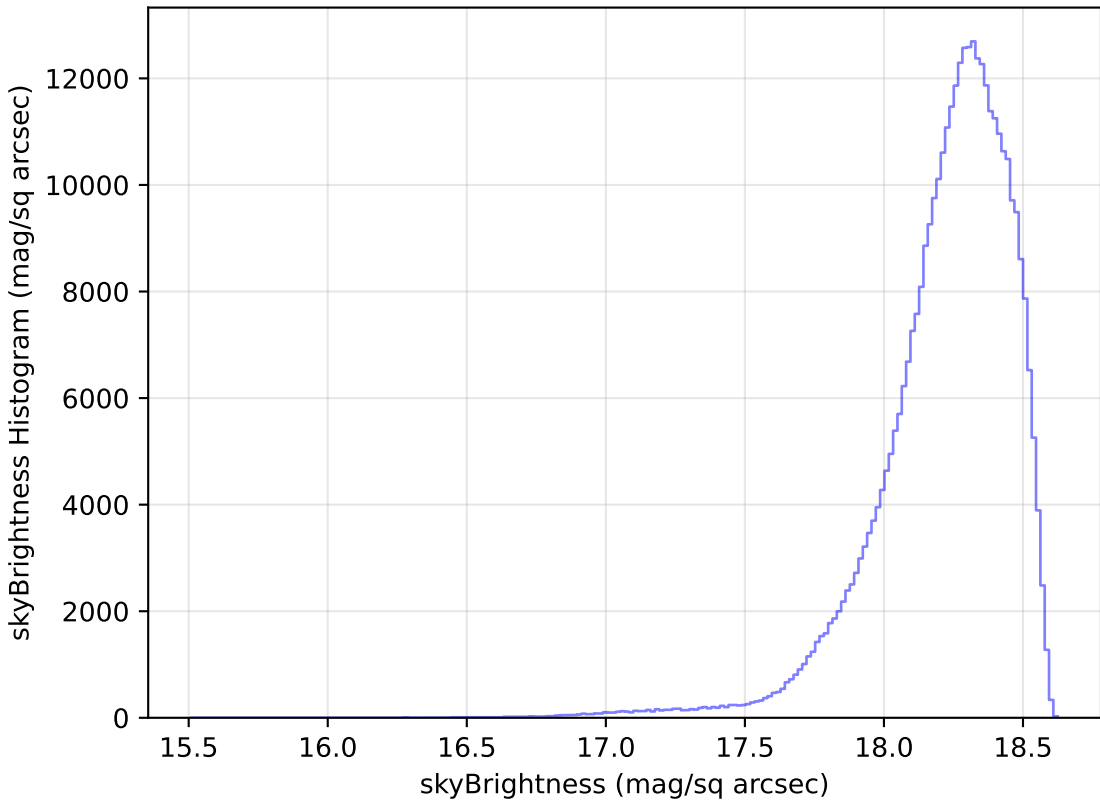
ddf_loaded_fl2_v3.4_10yrs WFD y band: skyBrightness Histogram
