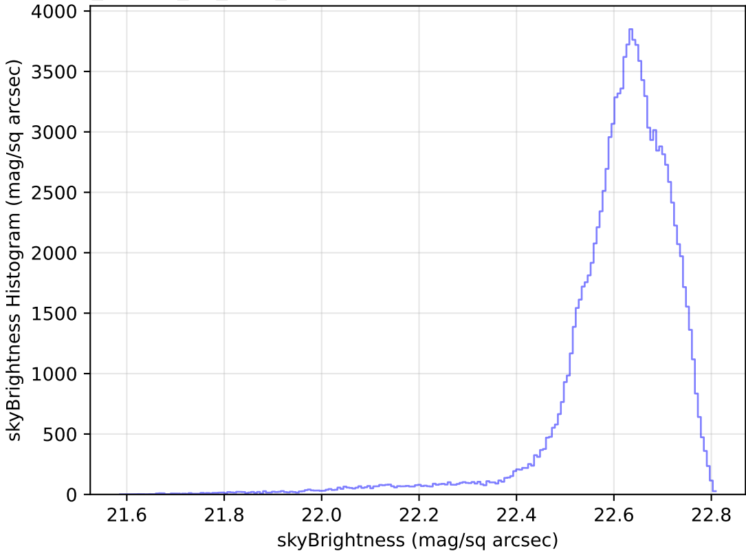
ddf_loaded_fl2_v3.4_10yrs WFD u band: skyBrightness Histogram
