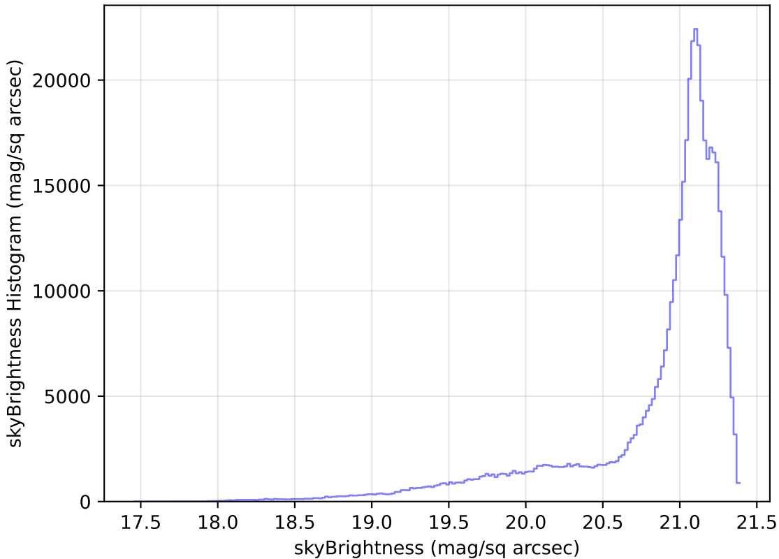
ddf_loaded_fl2_v3.4_10yrs WFD r band: skyBrightness Histogram
